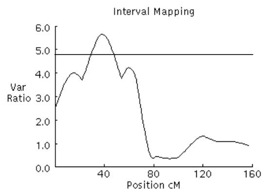
Figure 4. F-ratio curves for intramuscular fat on chromosome 8. The x-axis indicates the relative position on the linkage map. The y-axis represents the F-ratio. The horizontal line indicates the 5% chromosome-wide significance level from the permutation test.
