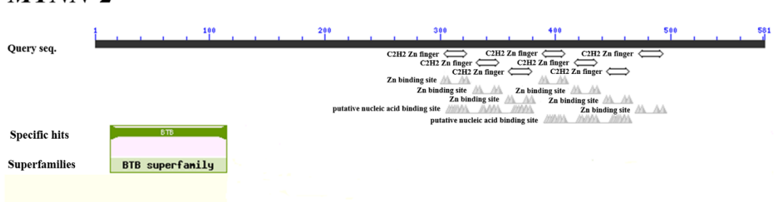
Figure S2. Conserved domain analysis of pig MYNN protein
