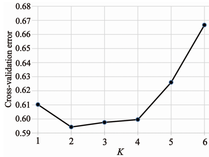
Supplementary Figure S1. Cross-validation error calculated for each value of K = 1 to 6 in ADMIXTURE program.
