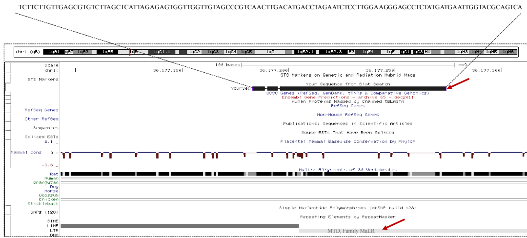
Figure S3. Blast result of transposon MTD .
