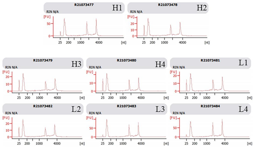
Figure S5. Electropherogram analysis of Total RNA on Agilent 2100 Bioanalyzer.
